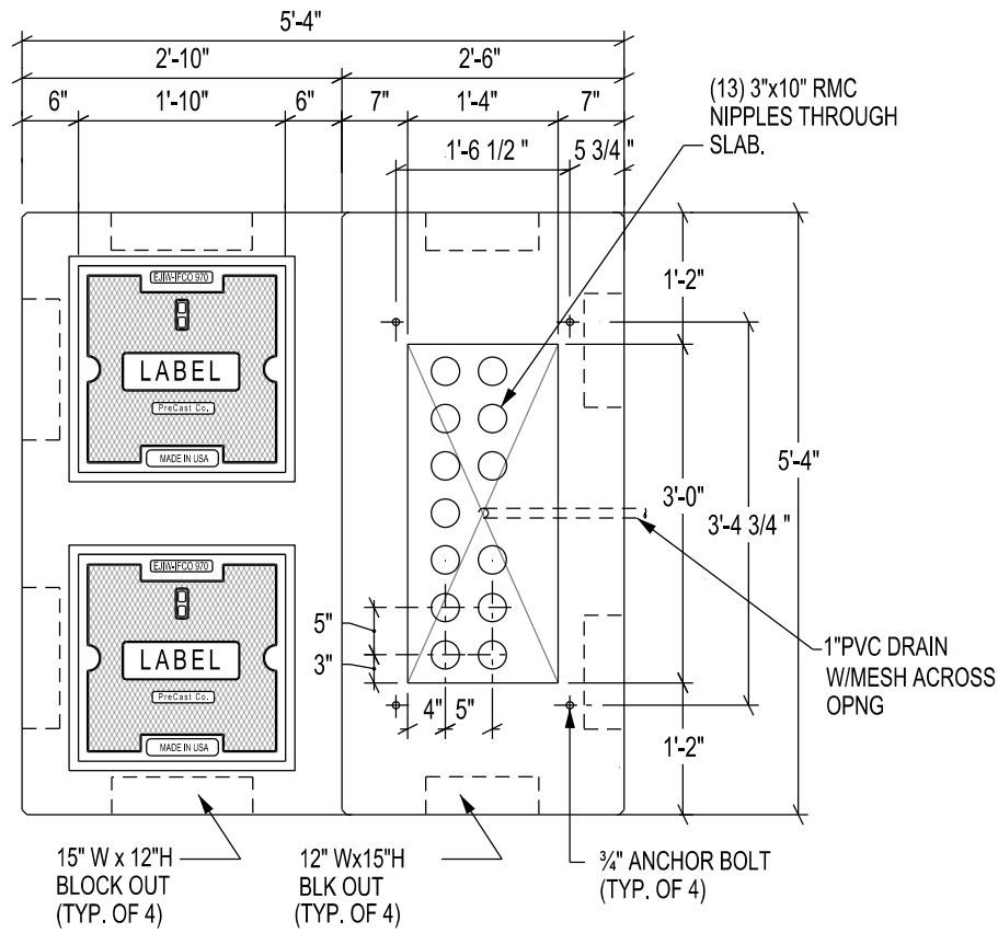
PLAN VIEW
