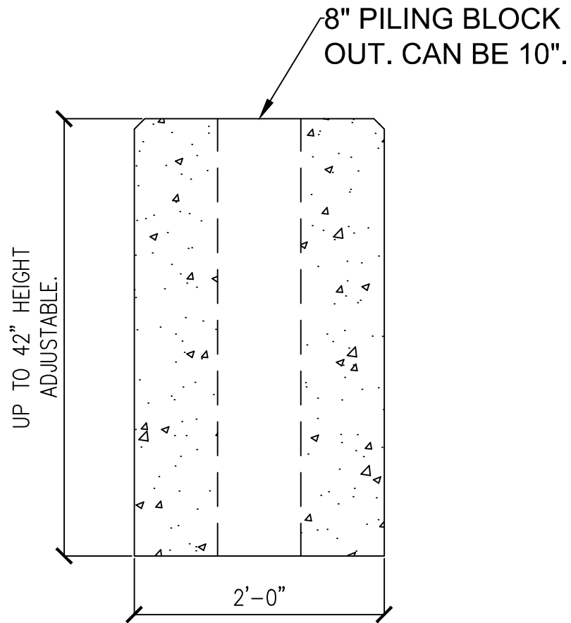
SECTION VIEW
