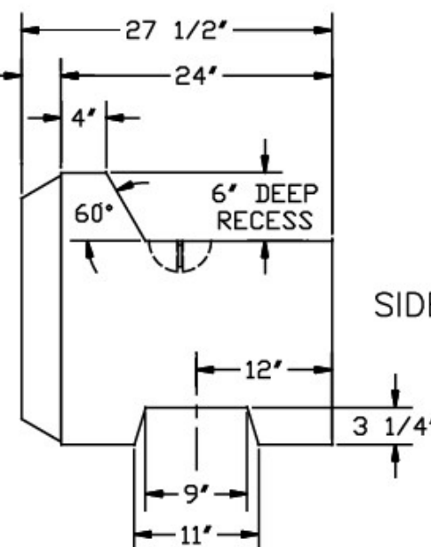
3 1/2" FORMLINER RELIEF
