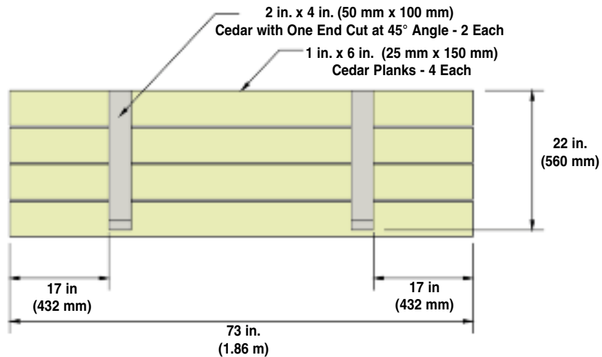
Figure 2: Seating Bench
