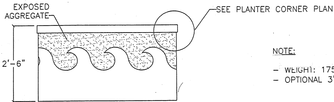
(A) 48" x 30" H (ID) WAVE PLANTER SCALE: \frac{1}{2}" = 1'
