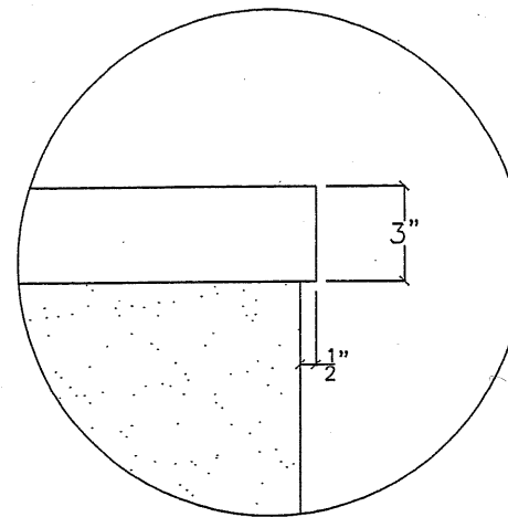
(C) PLANTER CORNER PLAN SCALE: NTS
