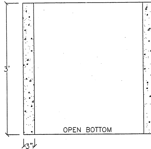
Ⓒ PLANTER SECTION PLAN SCALE: \frac{3}{4}''=1'
