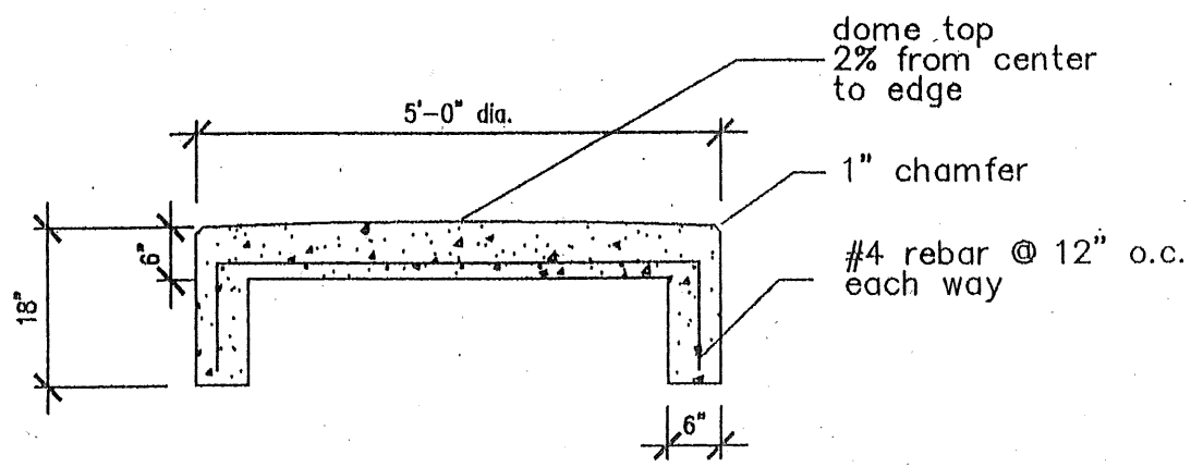
CROSS SCT.
